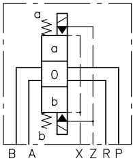
Manifold mounting valve
